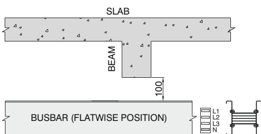
FIGURE-4 CROSSING UNDER A BEAM HORIZONTAL POSITION
